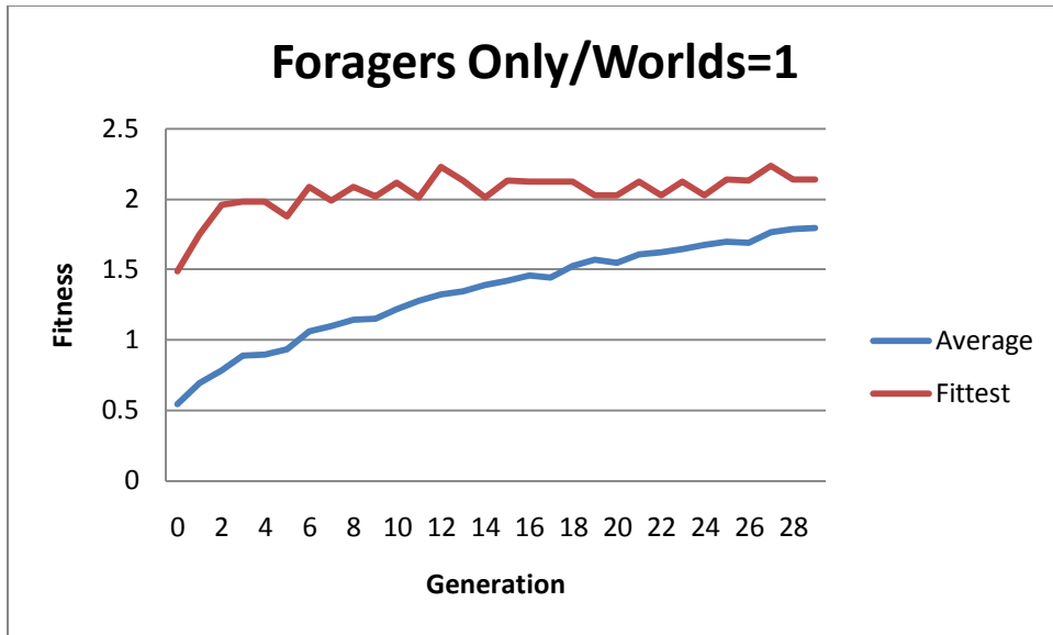
Figure 1 – Mox forager performance learning a single world
